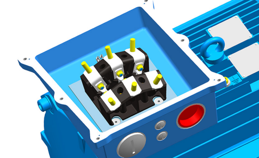
Terminal board for motor size 280 to 355.
