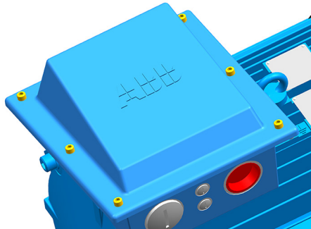
Terminal box for motors size 280 to 355.
